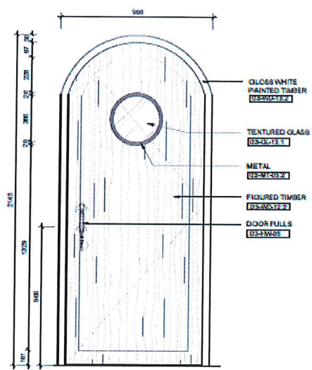
C ELEVATION
