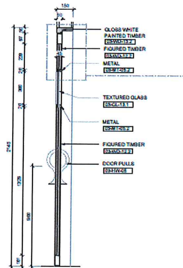
D SECTION
