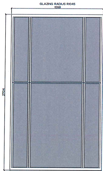
110 EXTERNAL ELEVATION
